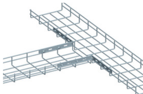
'T' Connector
